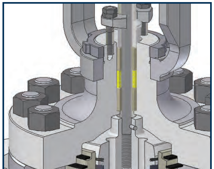
PACKING ARRANGEMENTS
