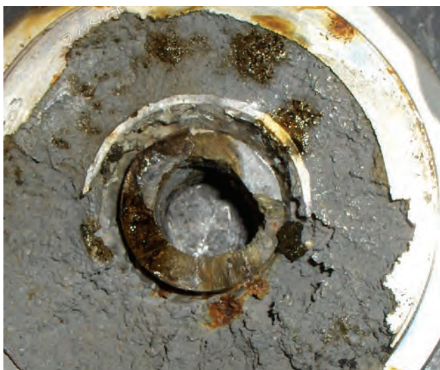
Typical cavitation damage
