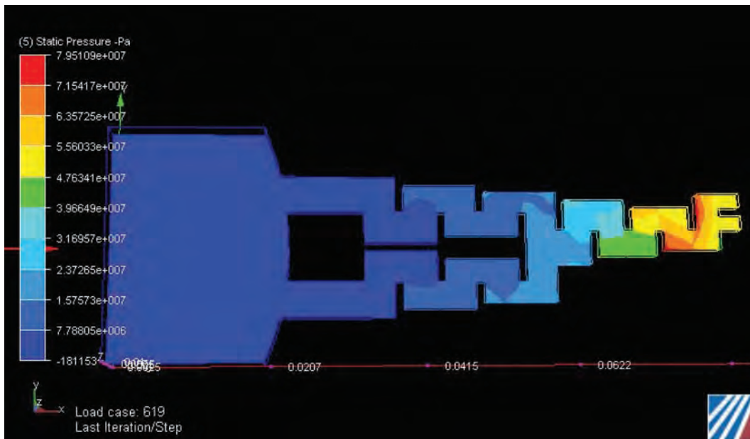
CFD analysis of a sectional VECTOR™ disc
